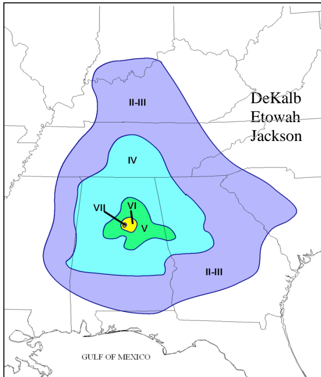
Figure 17: Isoseismic Map shows shaking intensities associated with the 5.1 magnitude Irontale earthquake in 1916. 6
